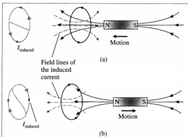
Lenz's law and Faraday's magnet and coil experiment. The solid curves in (a) and (b) are the lines of magnetic induction of the bar magnet and the dashed curves are those of the induced current.
