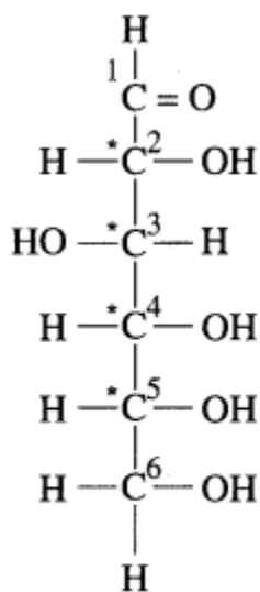
Structural formula of glucose
