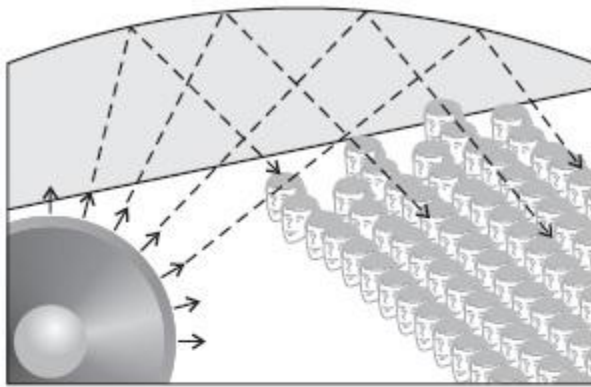
Fig. 12.14: Curved ceiling of a conference hall.
