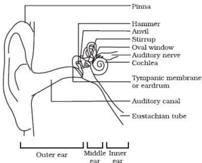
Fig. 12.19: Auditory parts of human ear.
