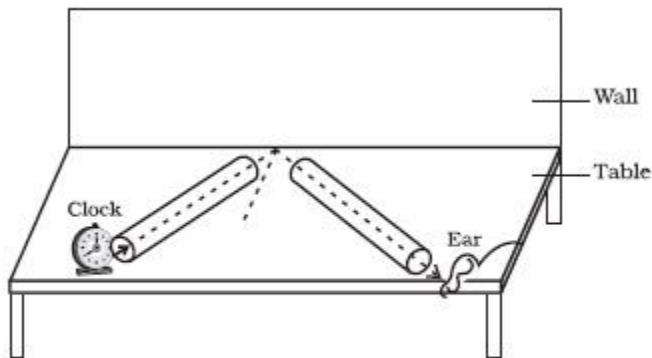
Fig. 12.11: Reflection of sound
