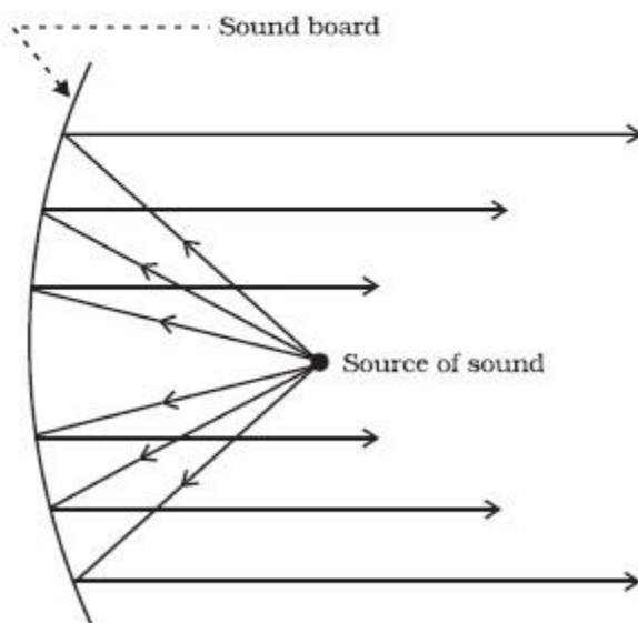
Fig. 12.15: Sound board used in a big hall.
