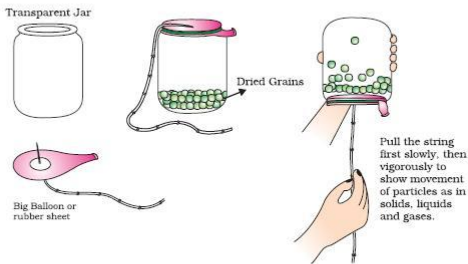
Fig. 1.10: A model for happy converting of solid to liquid and liquid to gas.
