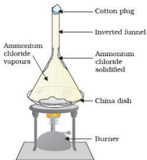
Fig. 1.7: Sublimation of ammonium chloride
