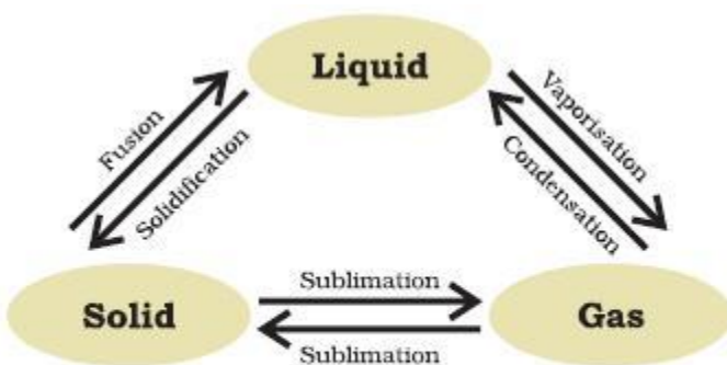
Fig. 1.9: Interconversion of the three states of matter
