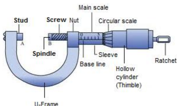
Diagram of screw gauge:
