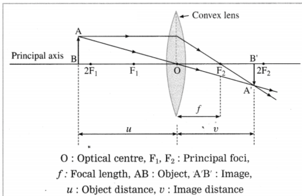
Object beyond 2F_1
