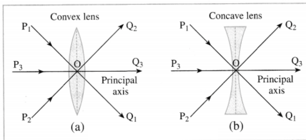
Fig. 7.5 : Optical centre of a lens
