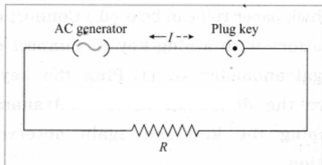
Fig. 4.27 (a) : Circuit
