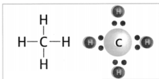
Structural formula and electron dot model of methane
