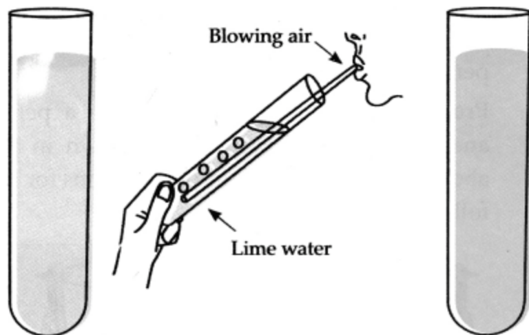
Reaction of limewater with \text{CO}_2
