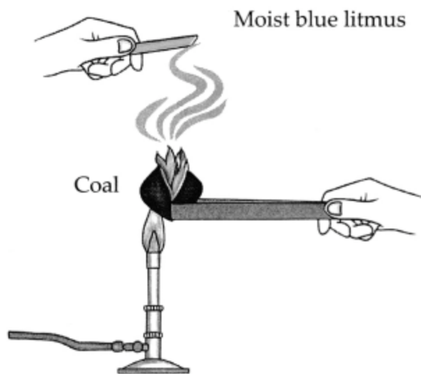
Reaction of carbon with oxygen
