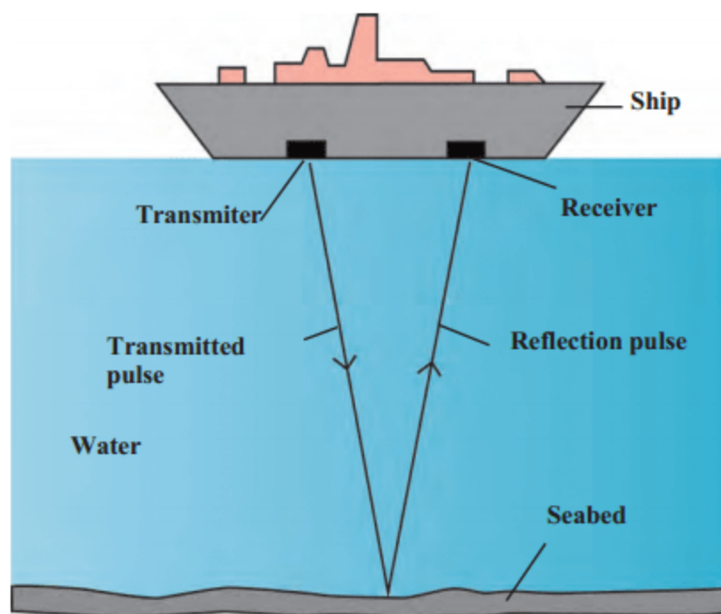
The SONAR technique
